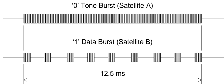
Figure 2: Timing Diagram for Tone Burst Control Signal
